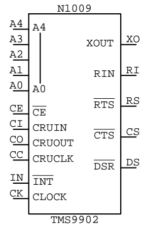
TMS9902
