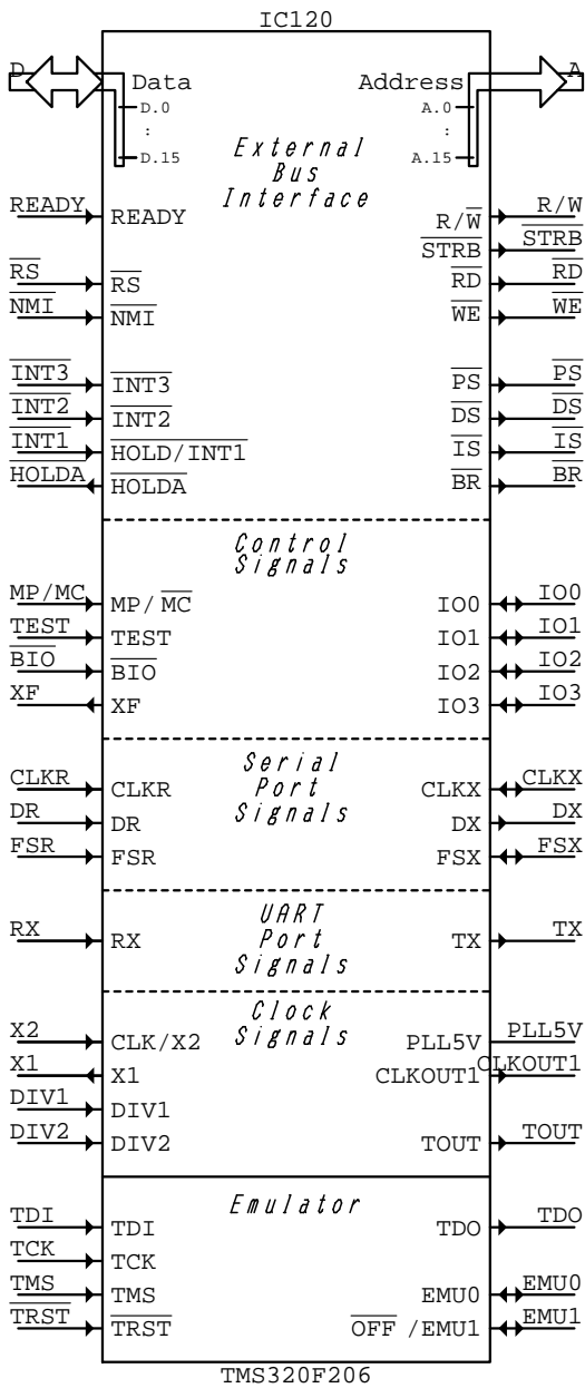
TMS320F206 IC???
