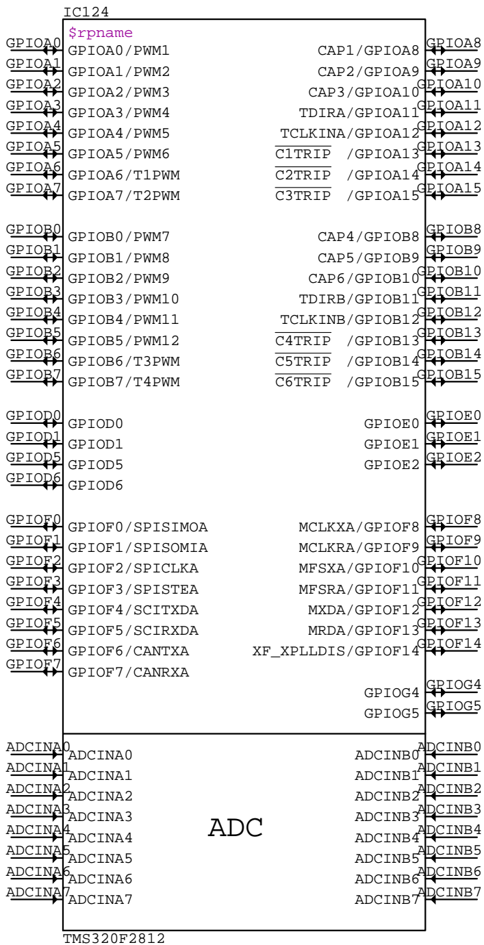
TMS320F2812_PORTS IC???
