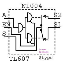
TL607 N????
