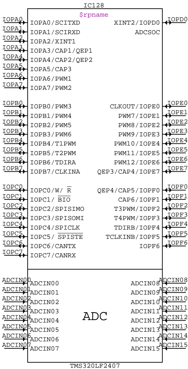
TMS320LF2407_PORTS
