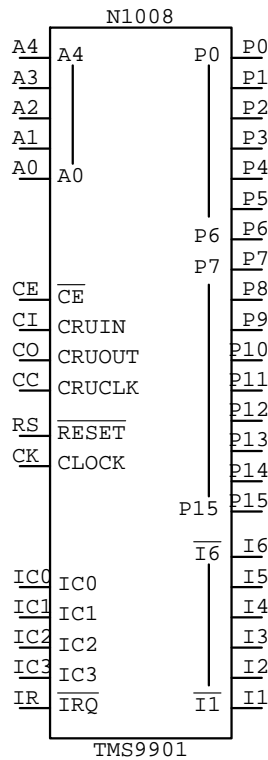
TMS9901
