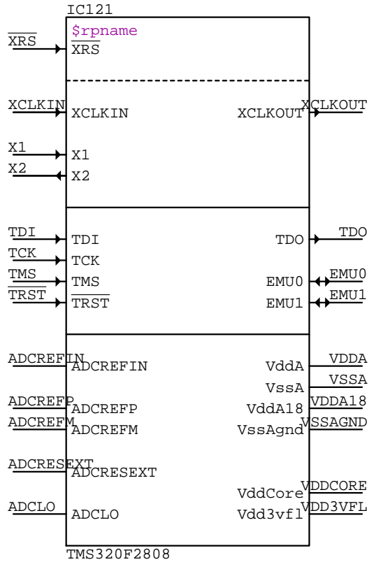
TMS320F2808 IC???
