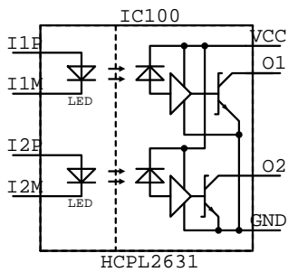
HCPL2631 IC???
