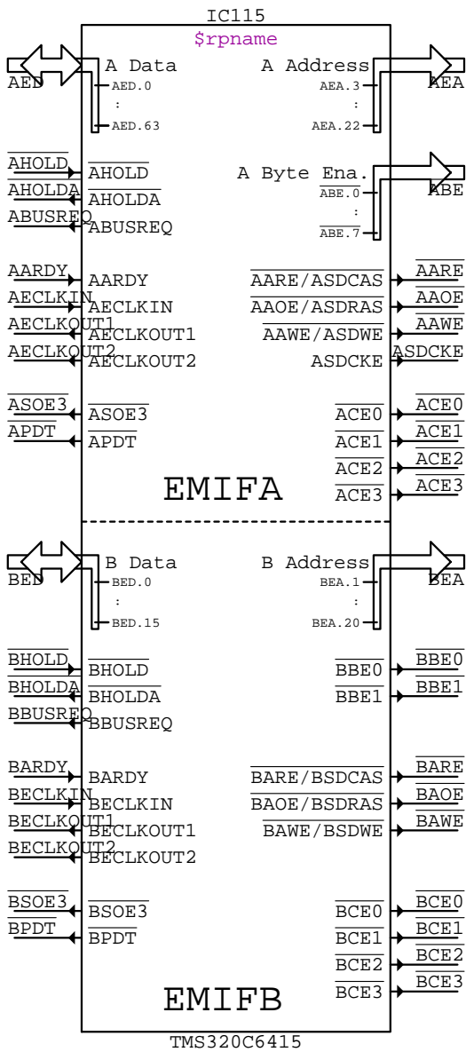
TMS320C6415_EMIF
