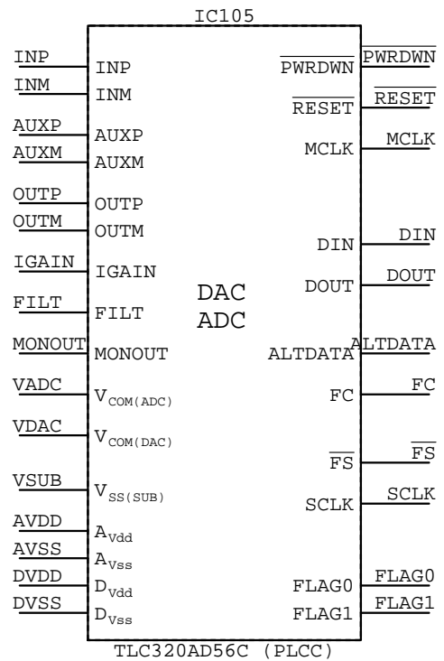
TLC320AD56CFN IC???
