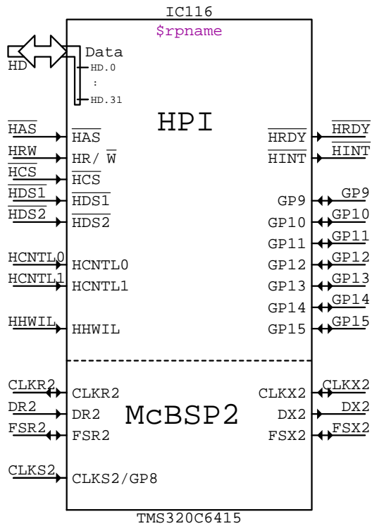
TMS320C6415_HPI
