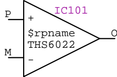
THS6022 IC???
