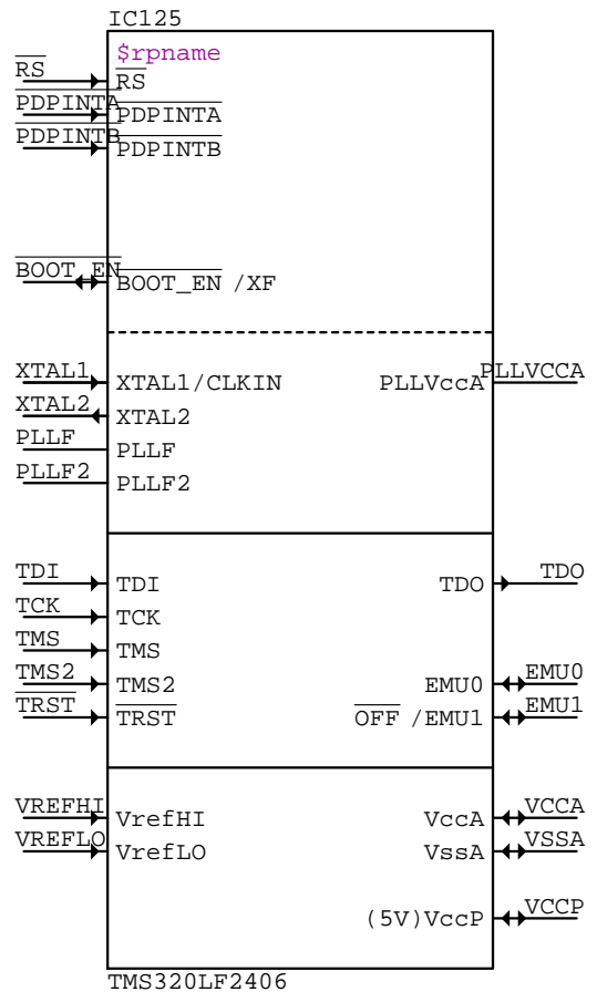
TMS320LF2406 IC???
