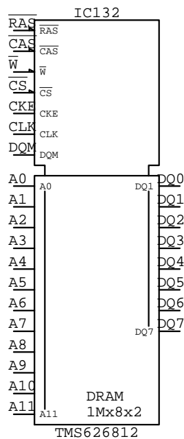
TMS626812 IC???
